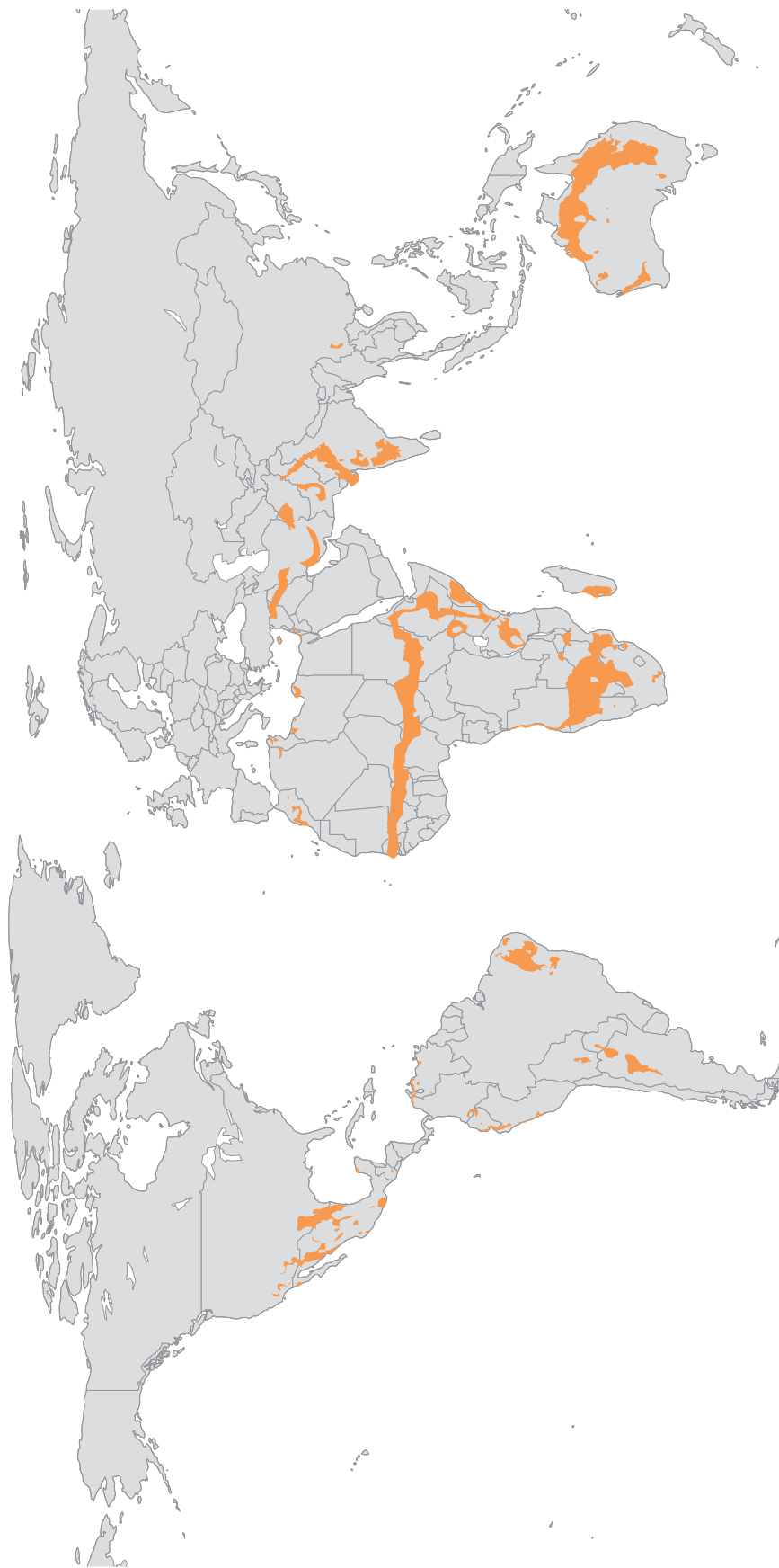
Main hot semi-arid environments of the world
