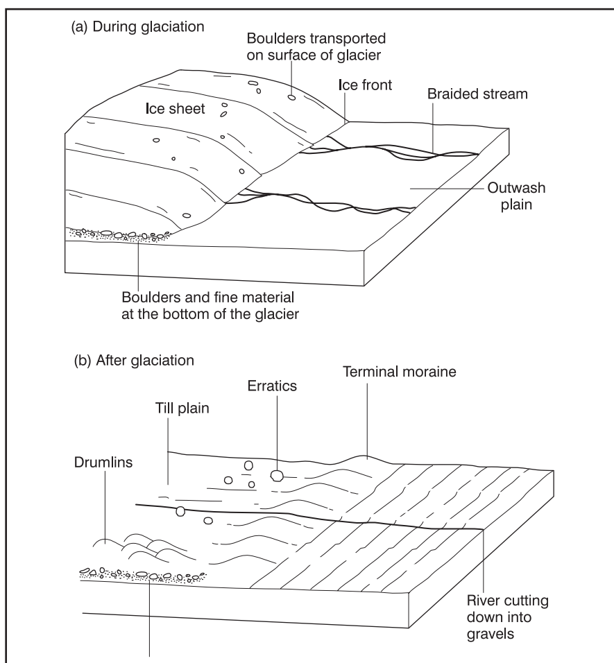
Figure 7: Before and after glaciation
