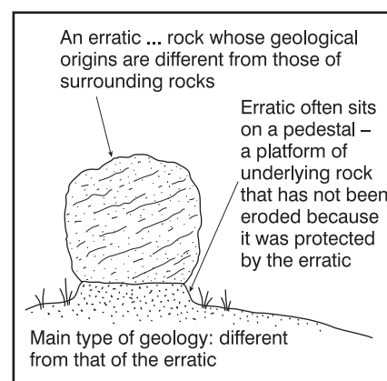
Figure 4: An erratic
