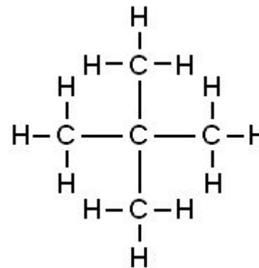
2,2-dimethylpropane
